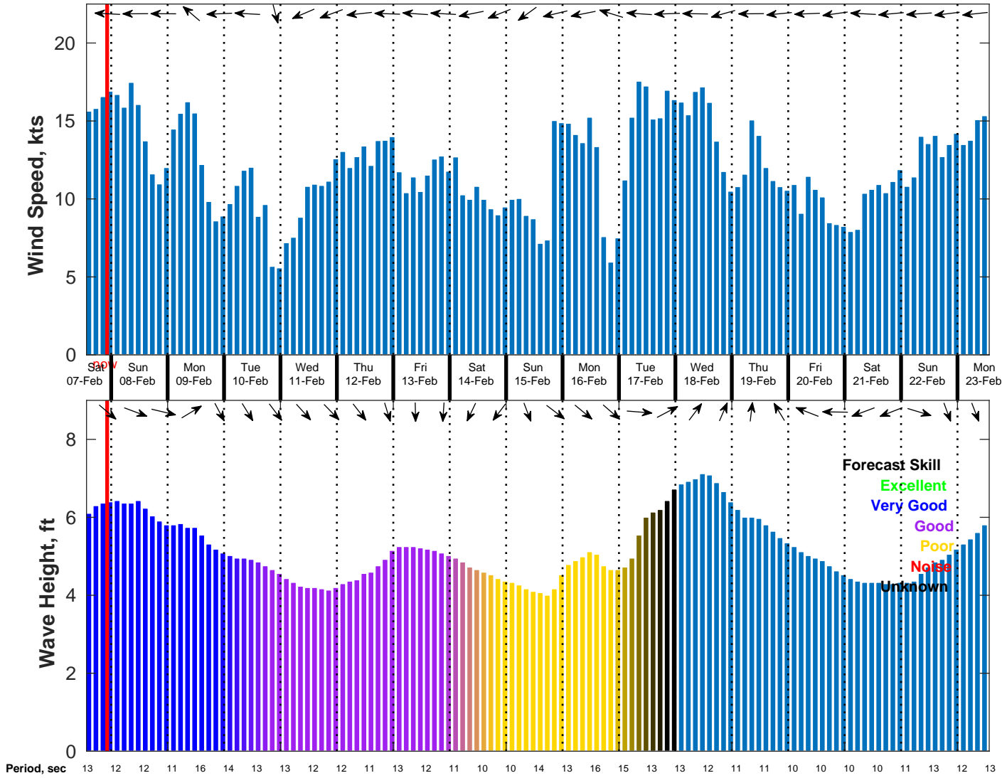
Wind & Wave Forecast for NDBC 51209 from 07-Feb-2026 13:00:00 to 23-Feb-2026 13:00:00
