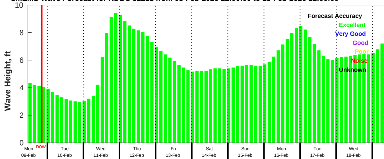
CMEMS Wave Forecast for NDBC 52211 from 08-Feb-2026 11:00:00 to 18-Feb-2026 11:00:00
