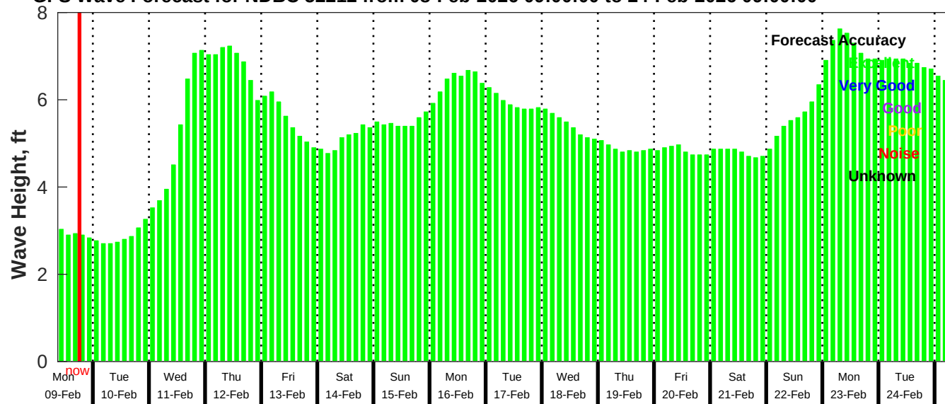
GFS Wave Forecast for NDBC 52212 from 08-Feb-2026 09:00:00 to 24-Feb-2026 09:00:00
