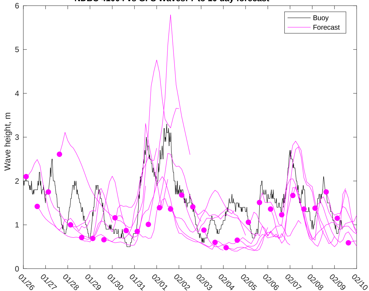
NDBC 41004 vs GFS Waves: 7 to 10 day forecast
