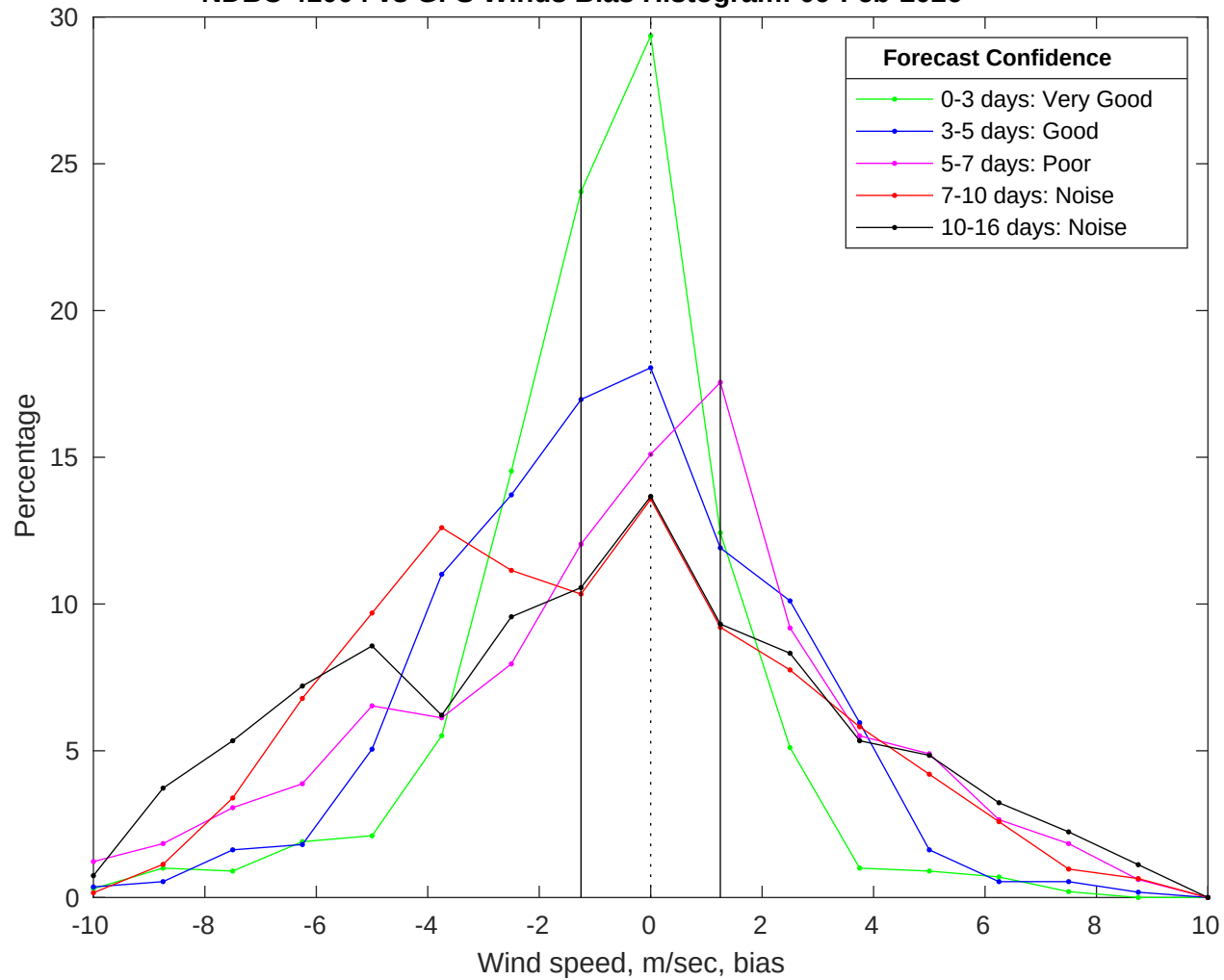
NDBC 41004 vs GFS Winds Bias Histogram: 09-Feb-2026
