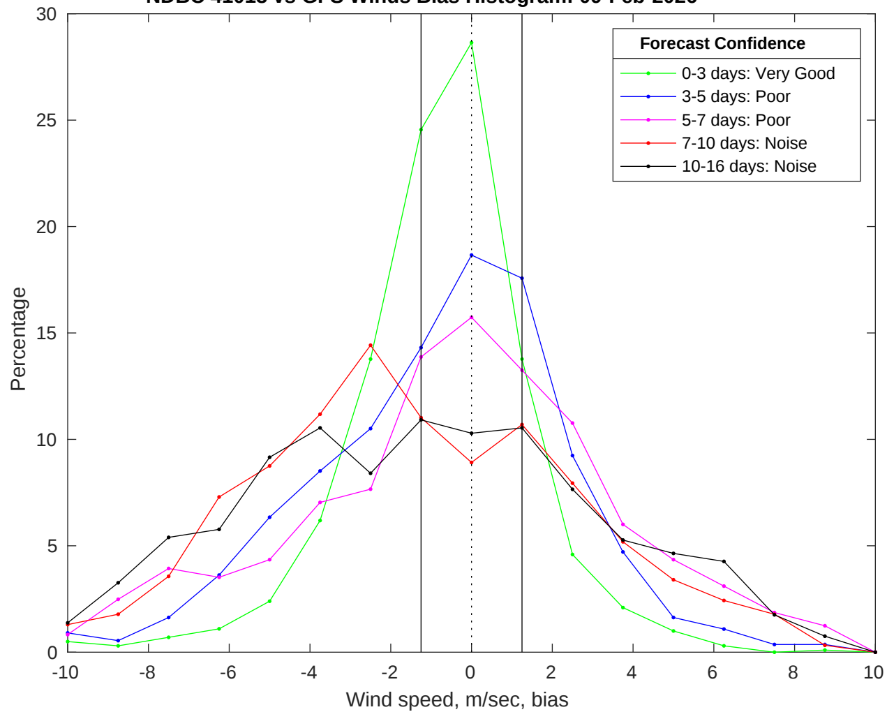
NDBC 41013 vs GFS Winds Bias Histogram: 09-Feb-2026
