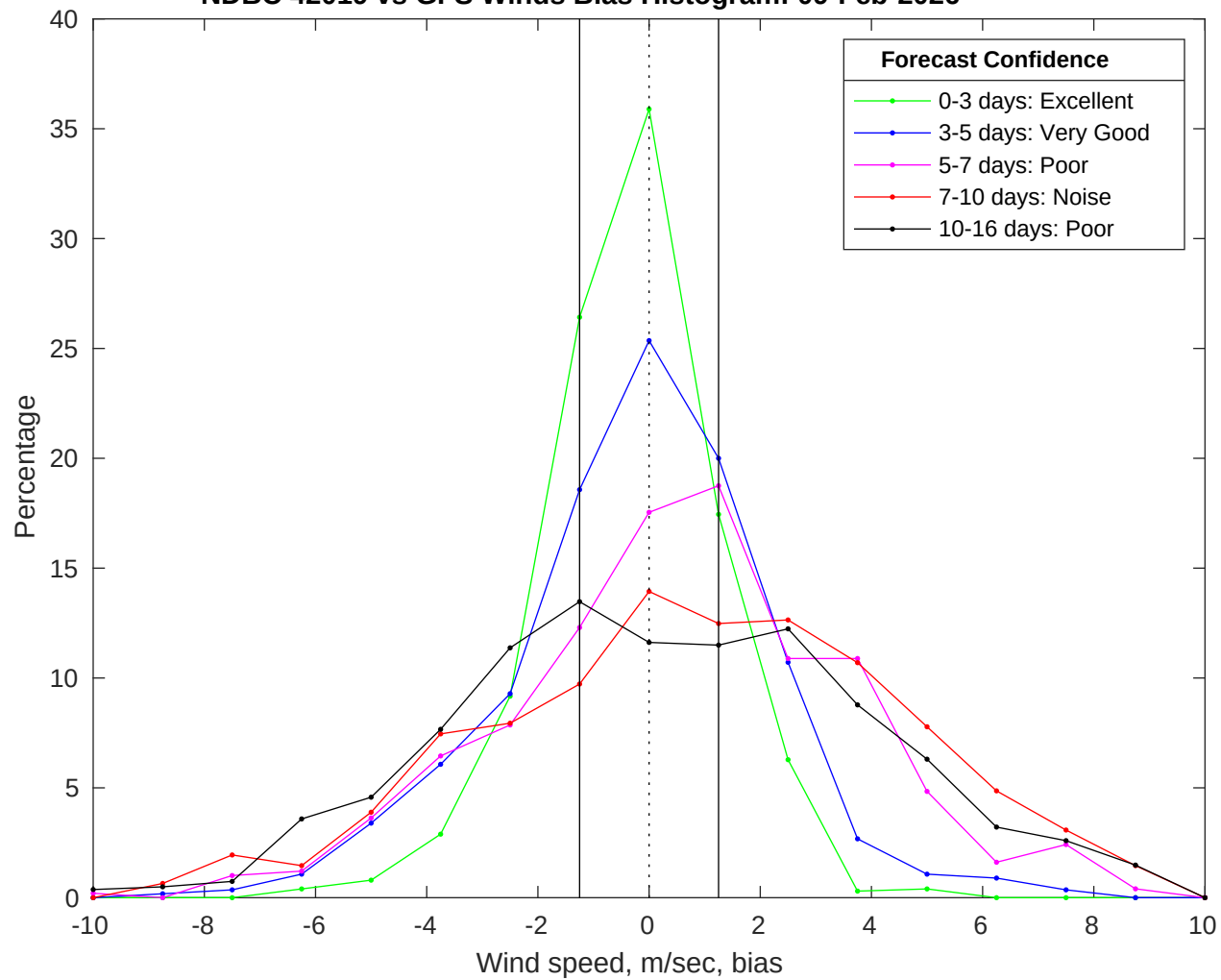
NDBC 42019 vs GFS Winds Bias Histogram: 09-Feb-2026
