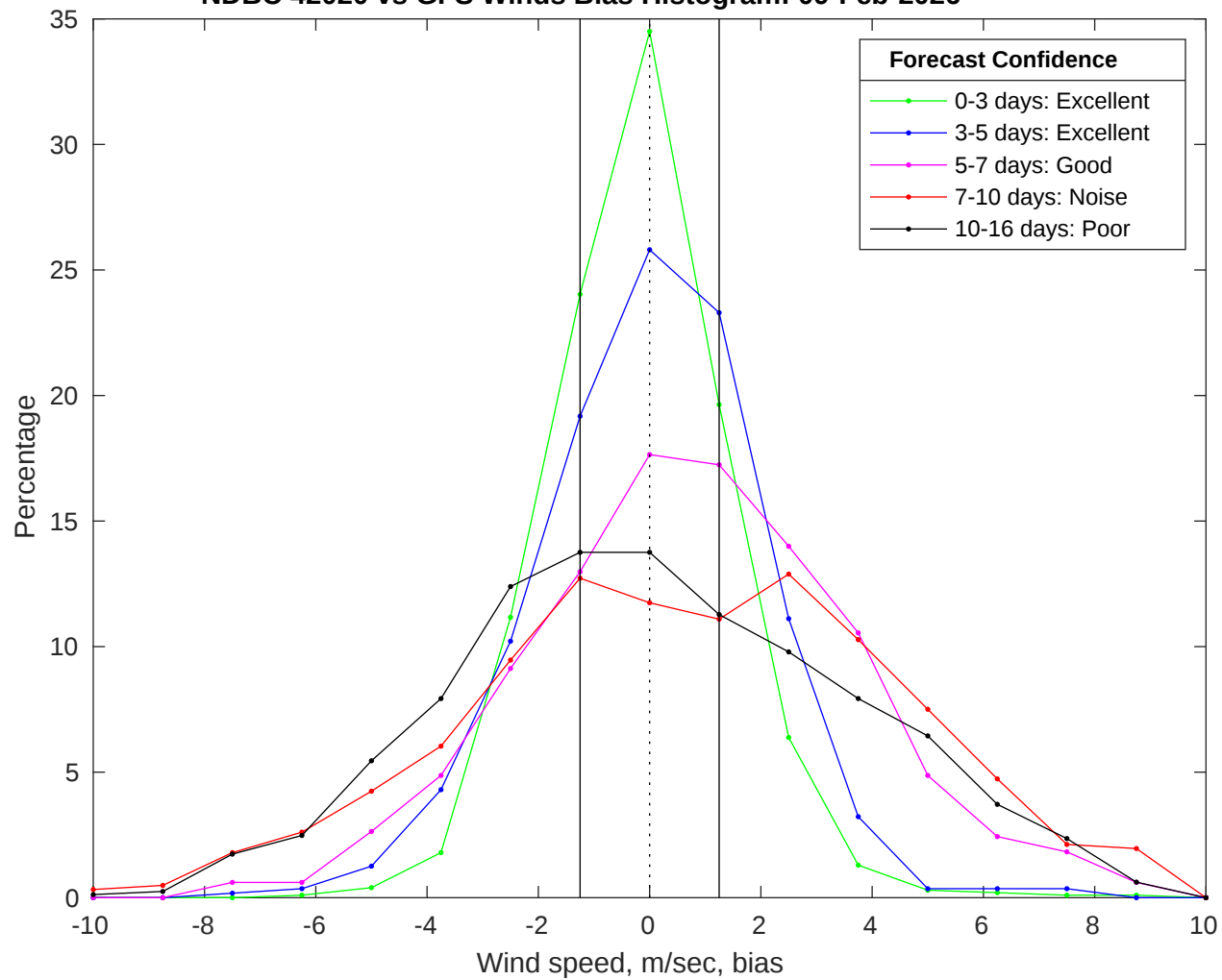
NDBC 42020 vs GFS Winds Bias Histogram: 09-Feb-2026
