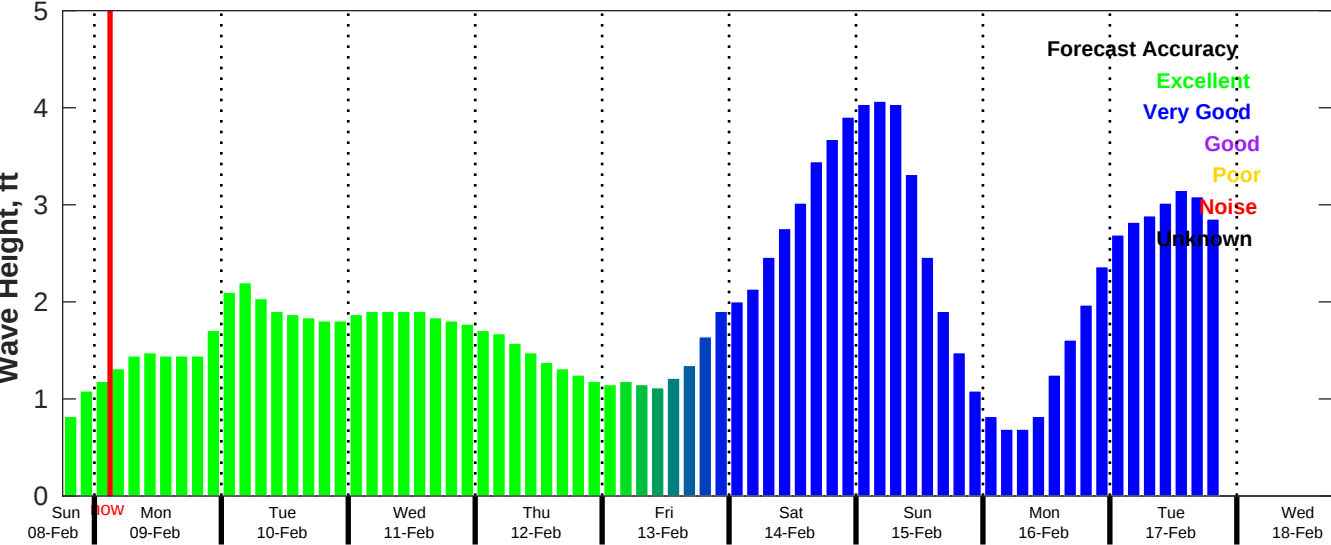
CMEMS Wave Forecast for NDBC 42035 from 08-Feb-2026 18:00:00 to 18-Feb-2026 18:00:00
