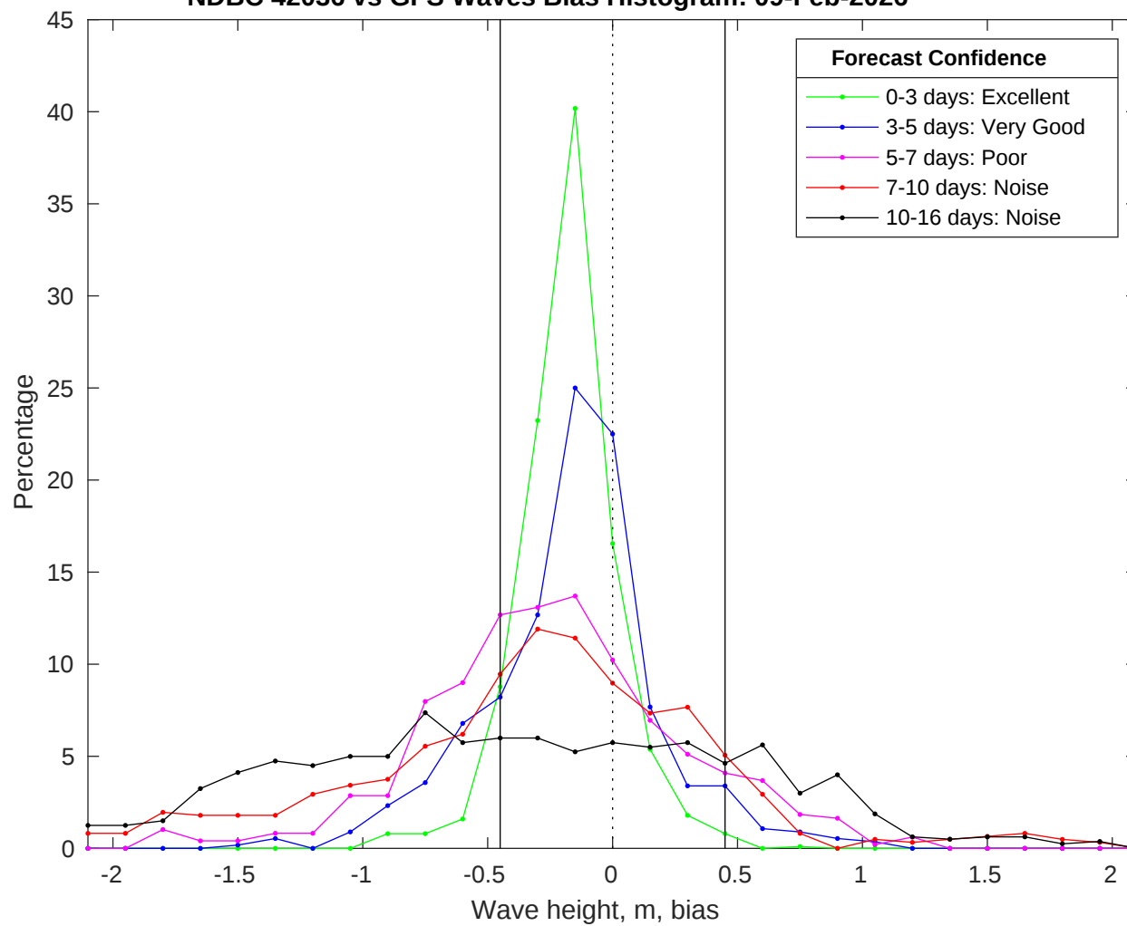
NDBC 42036 vs GFS Waves Bias Histogram: 09-Feb-2026
