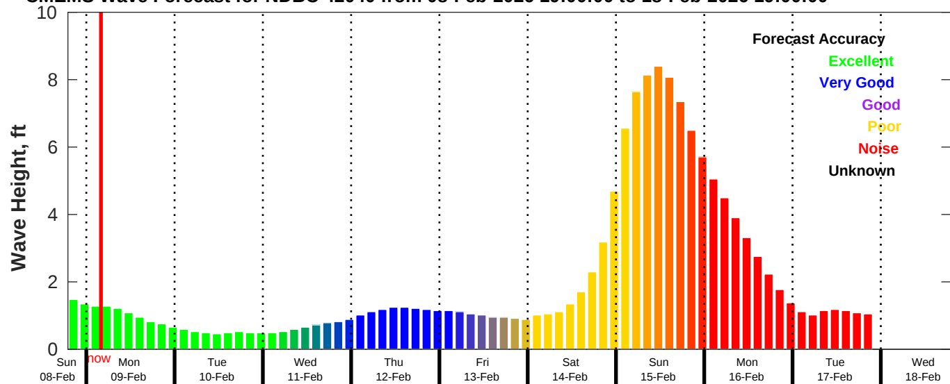
CMEMS Wave Forecast for NDBC 42040 from 08-Feb-2026 19:00:00 to 18-Feb-2026 19:00:00
