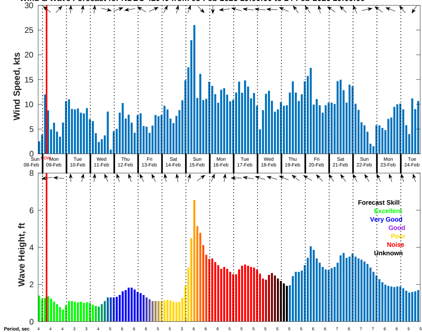
Wind & Wave Forecast for NDBC 42040 from 08-Feb-2026 19:00:00 to 24-Feb-2026 19:00:00
