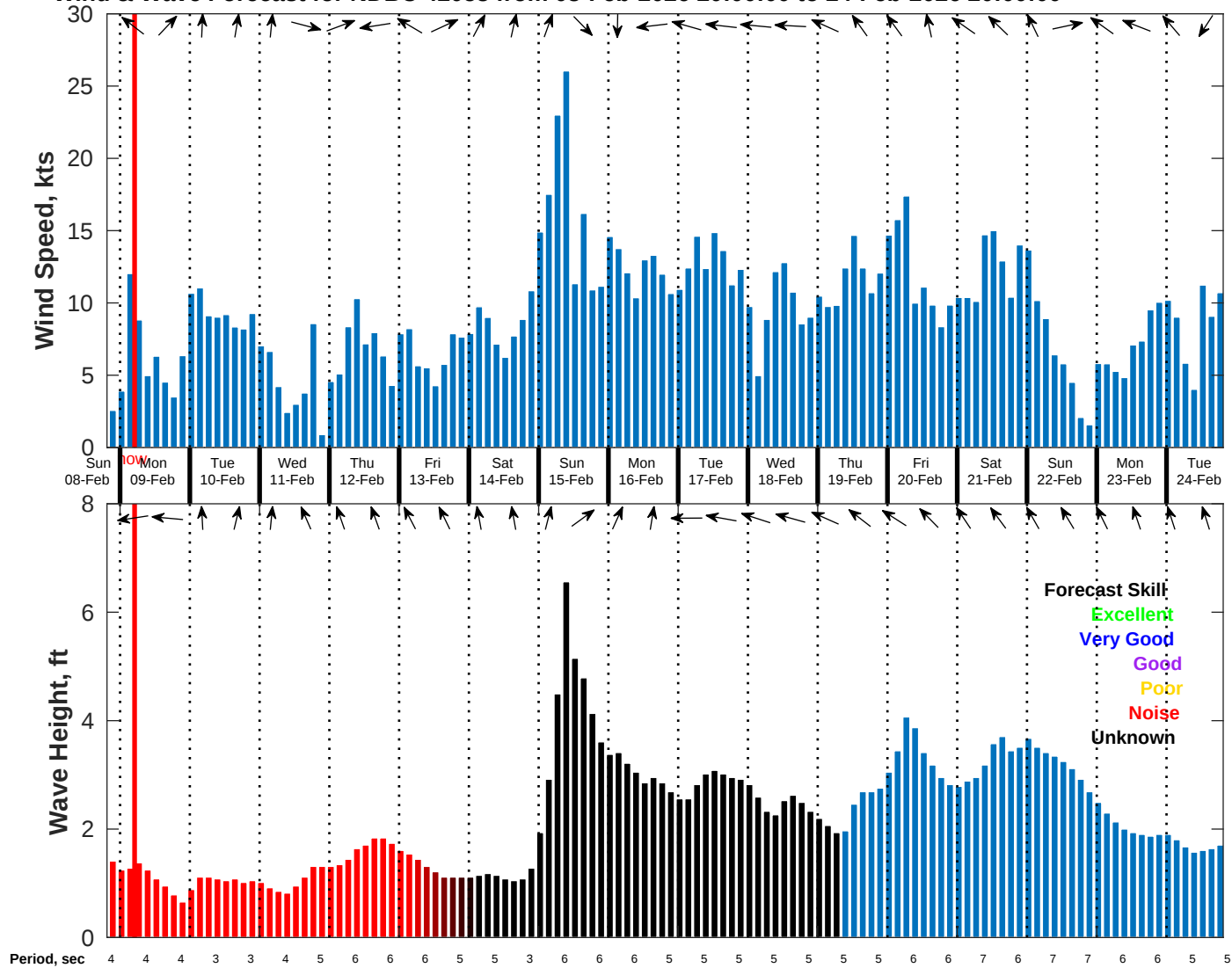
Wind & Wave Forecast for NDBC 42058 from 08-Feb-2026 20:00:00 to 24-Feb-2026 20:00:00
