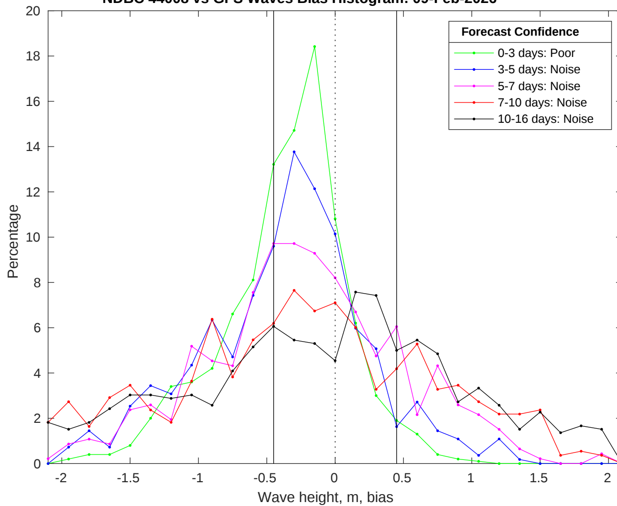
NDBC 44008 vs GFS Waves Bias Histogram: 09-Feb-2026
