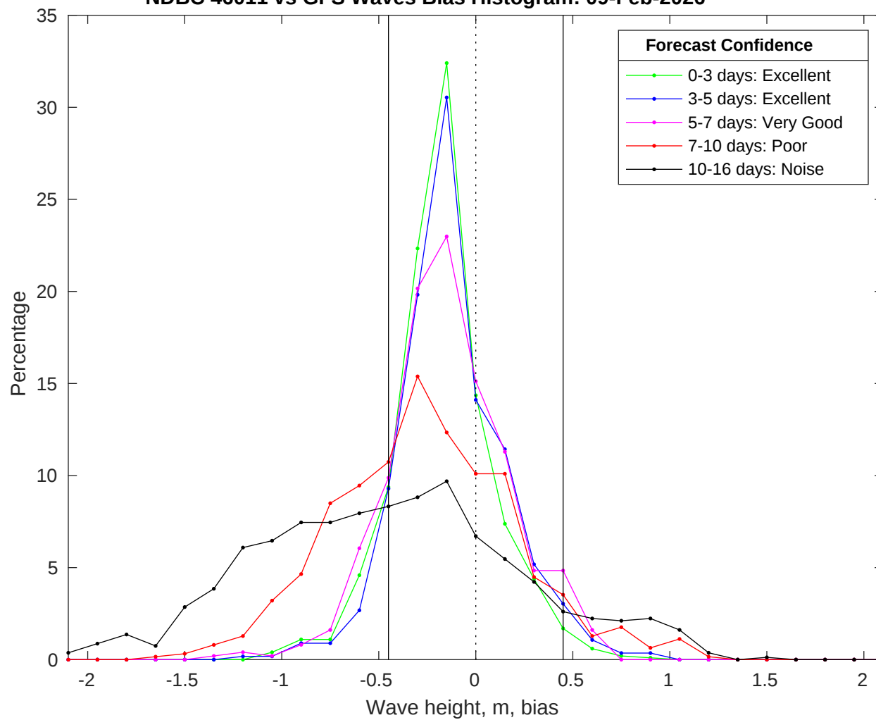
NDBC 46011 vs GFS Waves Bias Histogram: 09-Feb-2026
