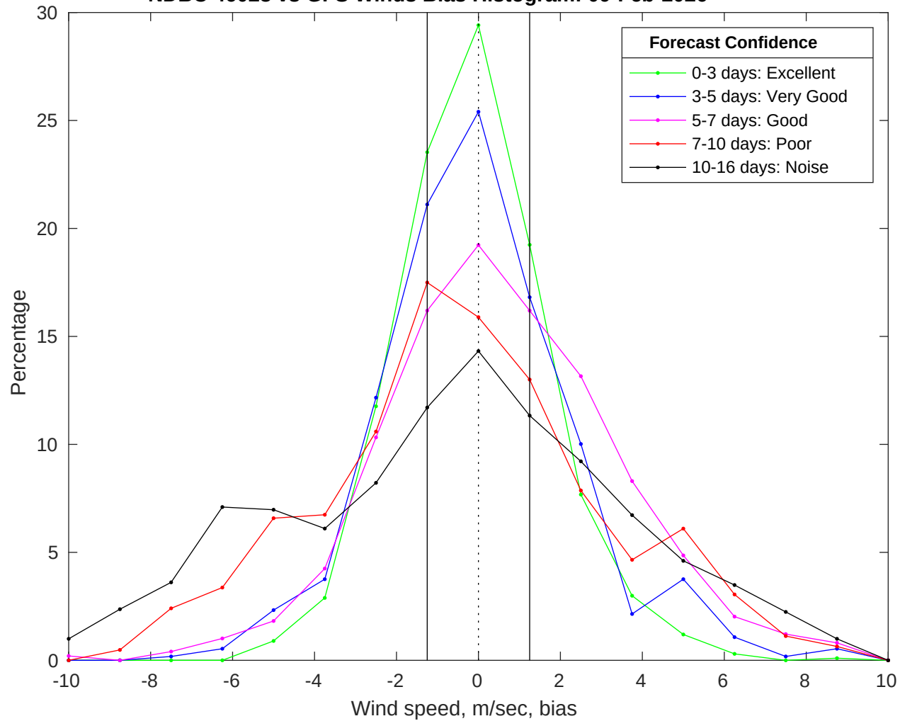
NDBC 46028 vs GFS Winds Bias Histogram: 09-Feb-2026
