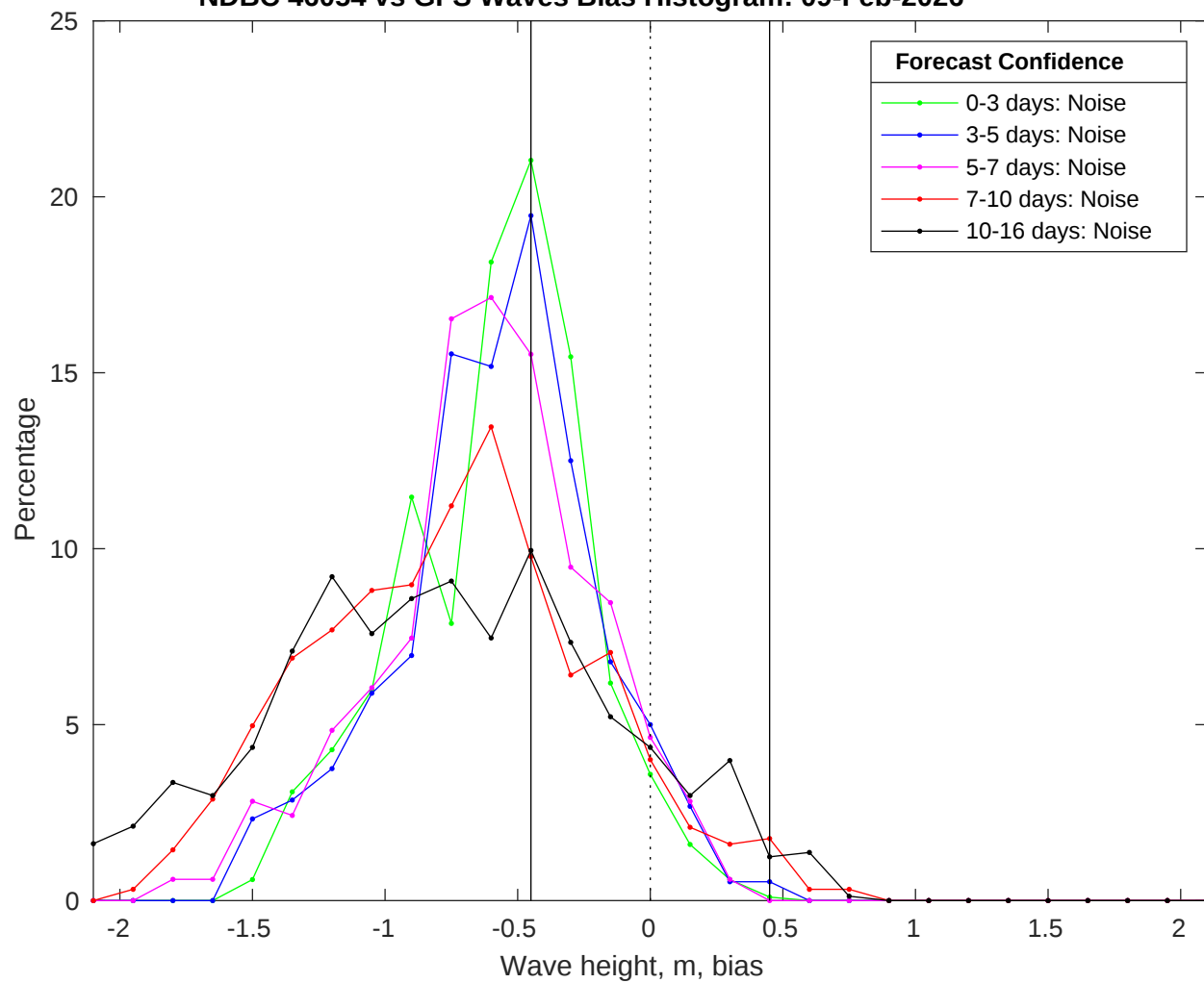
NDBC 46054 vs GFS Waves Bias Histogram: 09-Feb-2026
