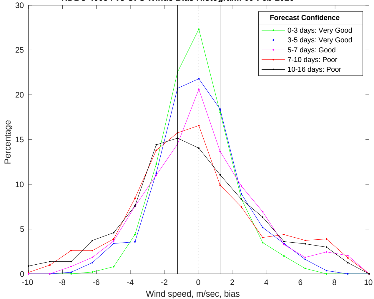
NDBC 46054 vs GFS Winds Bias Histogram: 09-Feb-2026
