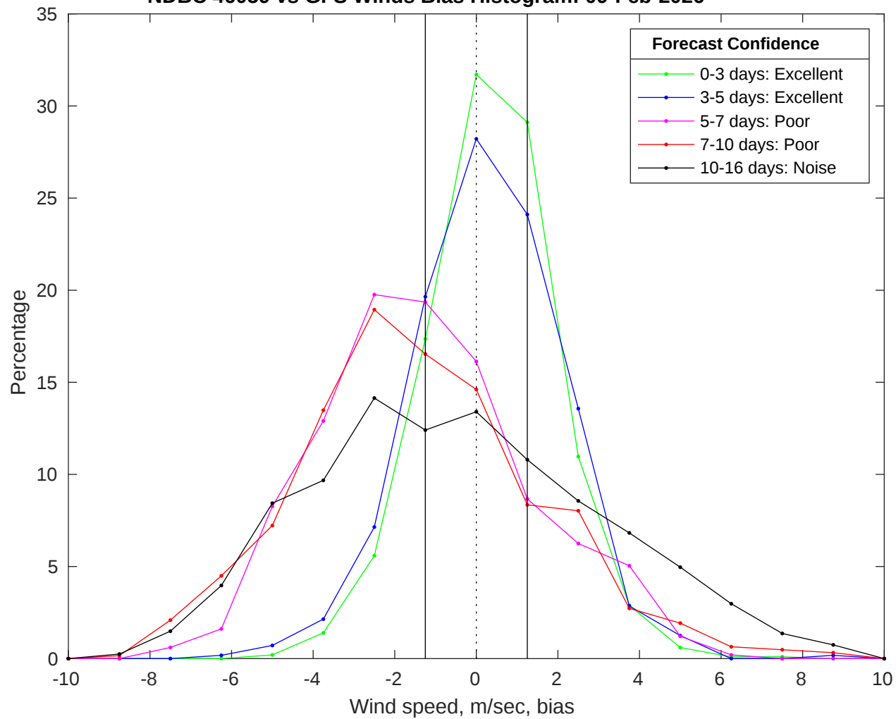
NDBC 46059 vs GFS Winds Bias Histogram: 09-Feb-2026
