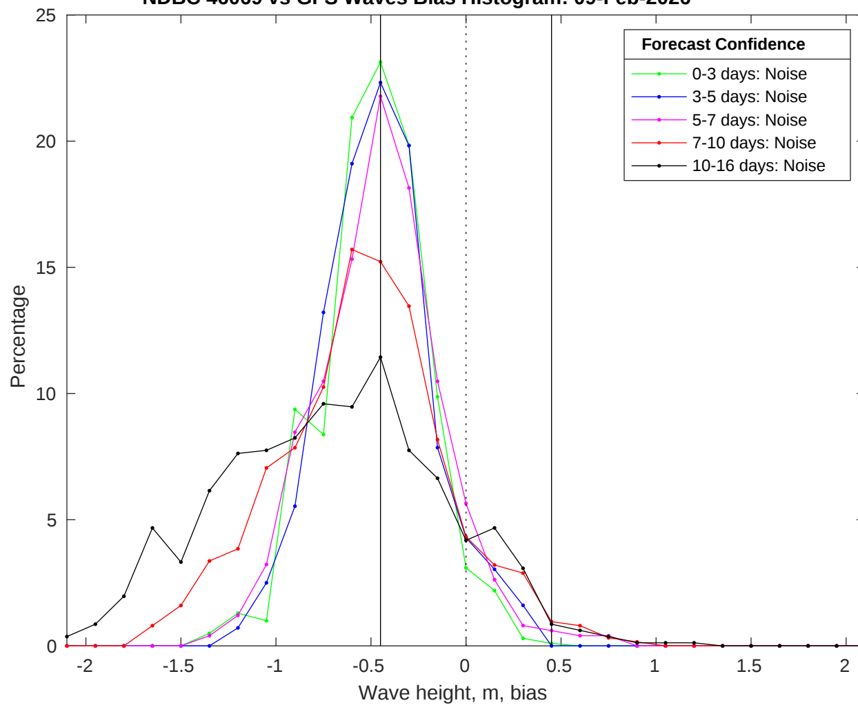
NDBC 46069 vs GFS Waves Bias Histogram: 09-Feb-2026
