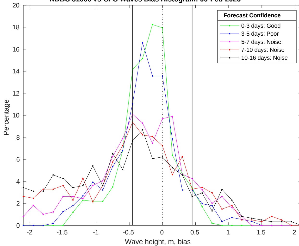
NDBC 51000 vs GFS Waves Bias Histogram: 09-Feb-2026
