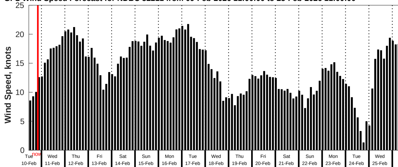
GFS Wind Speed Forecast for NDBC 52211 from 09-Feb-2026 11:00:00 to 25-Feb-2026 11:00:00
