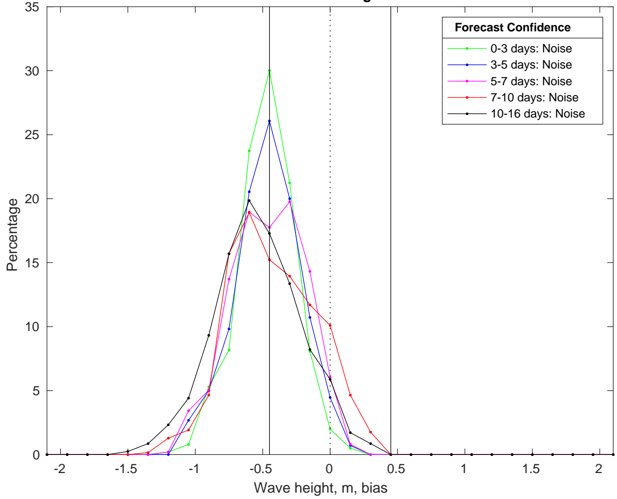
NDBC 52213 vs GFS Waves Bias Histogram: 09-Feb-2026
