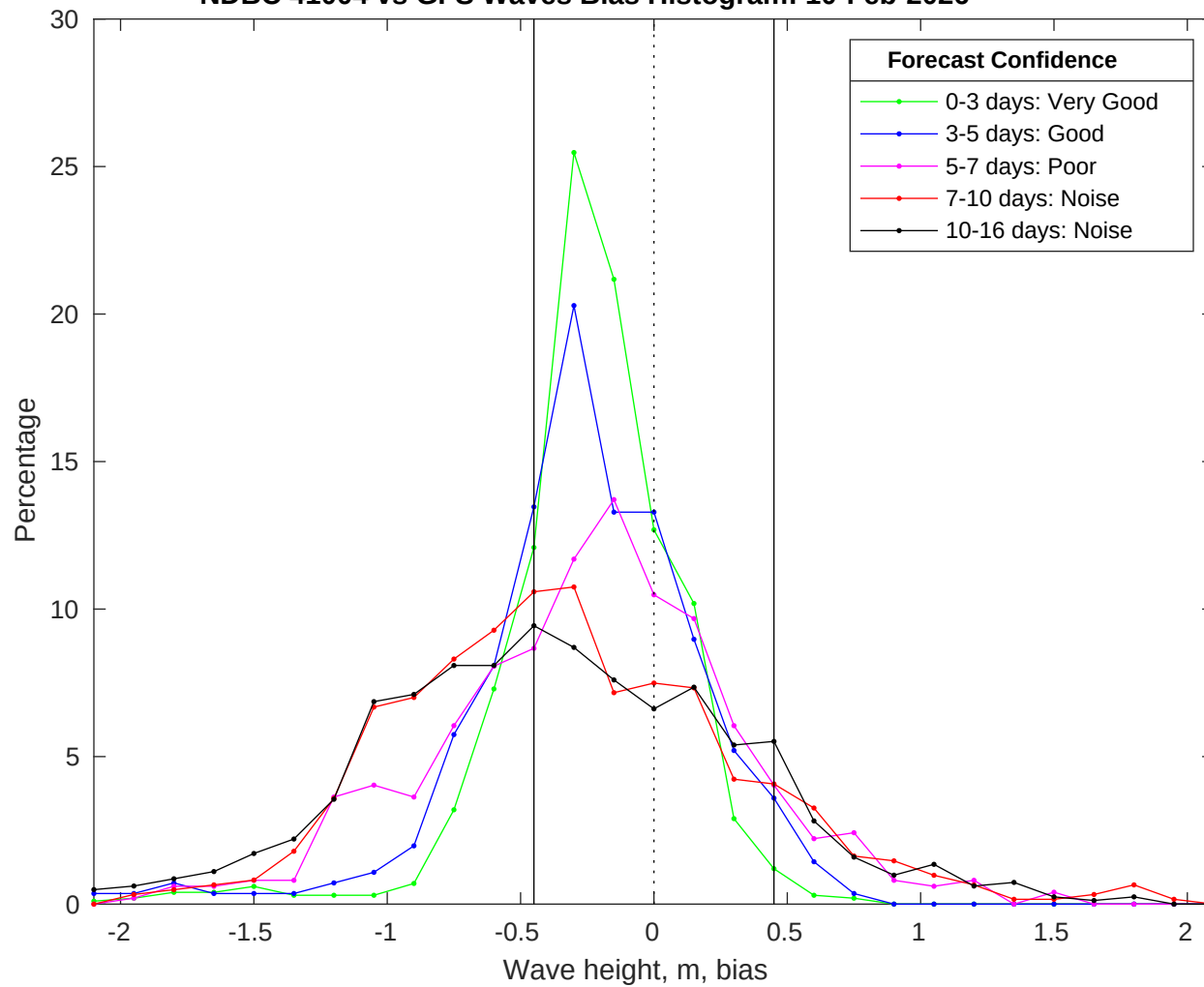
NDBC 41004 vs GFS Waves Bias Histogram: 10-Feb-2026
