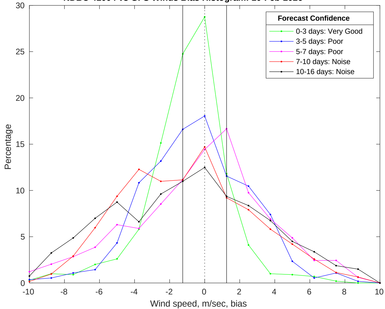
NDBC 41004 vs GFS Winds Bias Histogram: 10-Feb-2026
