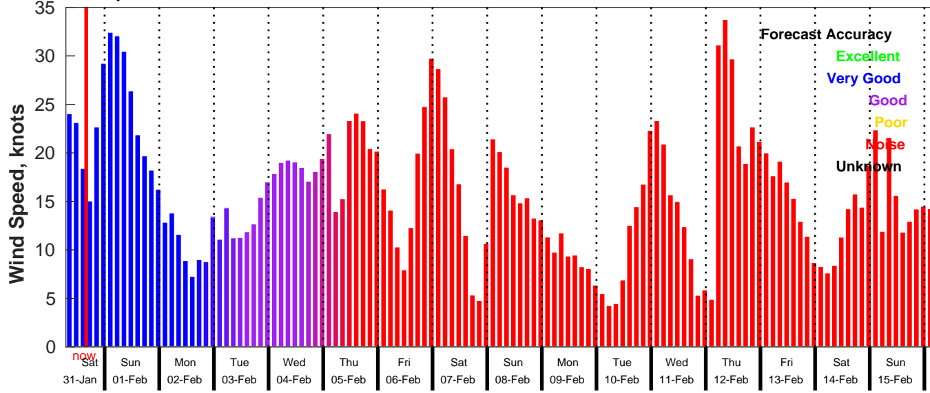
GFS Wind Speed Forecast for NDBC 41004 from 31-Jan-2026 07:00:00 to 16-Feb-2026 07:00:00
