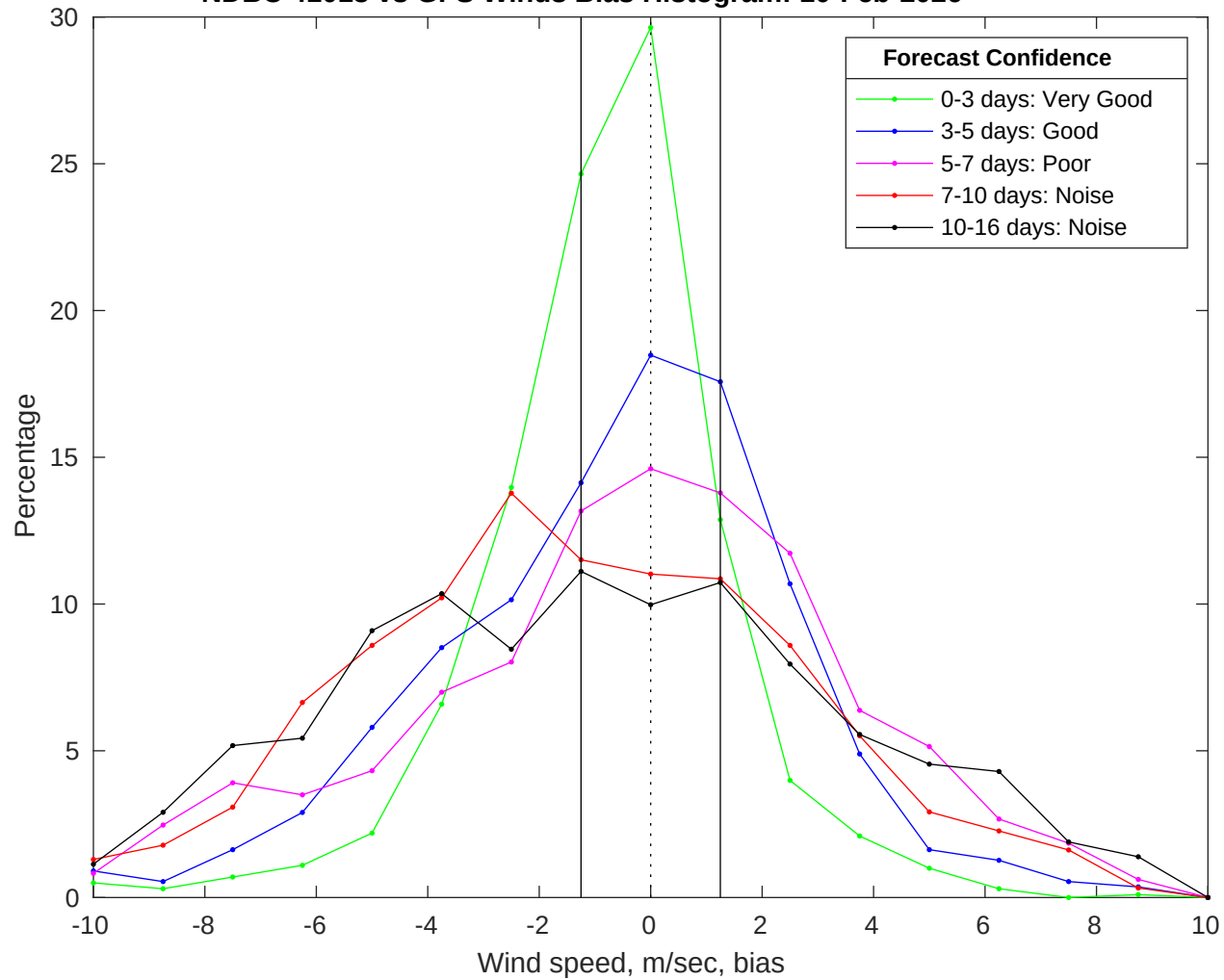
NDBC 41013 vs GFS Winds Bias Histogram: 10-Feb-2026
