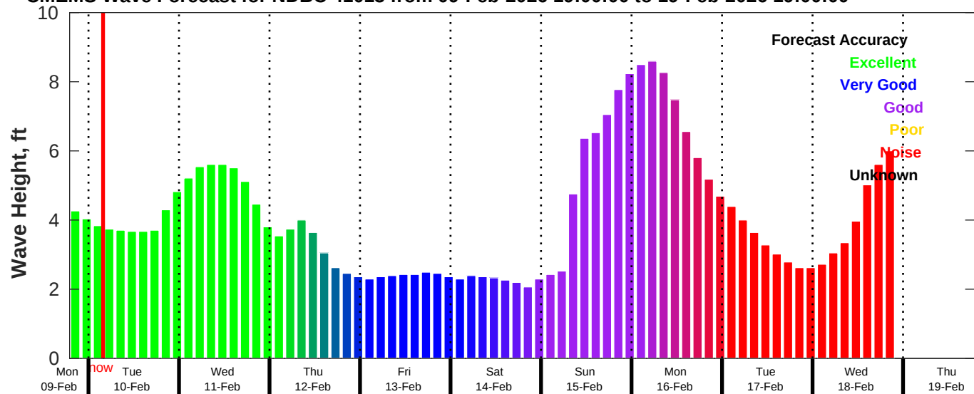
CMEMS Wave Forecast for NDBC 41013 from 09-Feb-2026 19:00:00 to 19-Feb-2026 19:00:00
