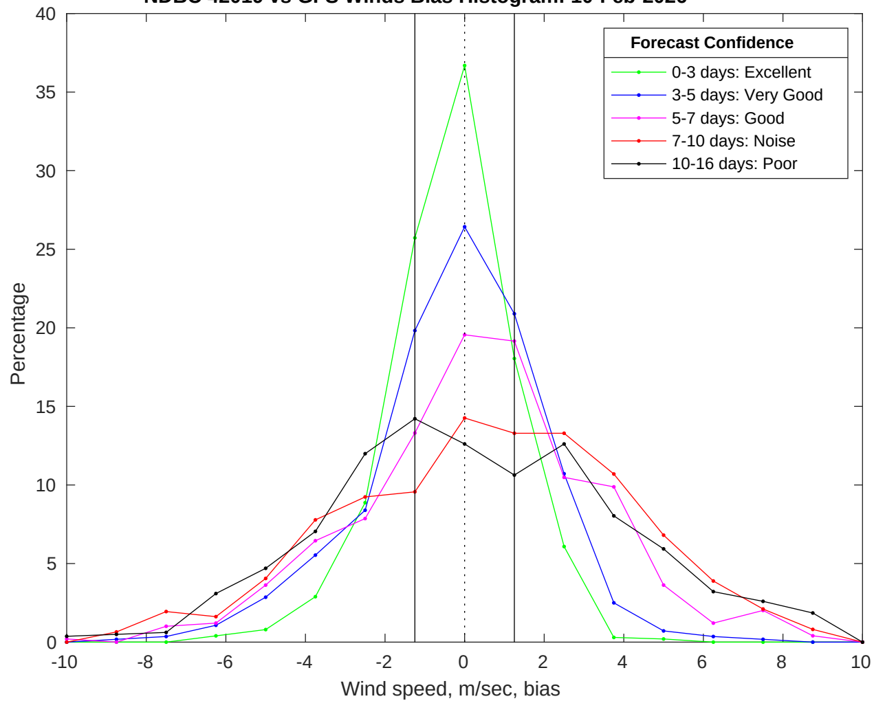
NDBC 42019 vs GFS Winds Bias Histogram: 10-Feb-2026
