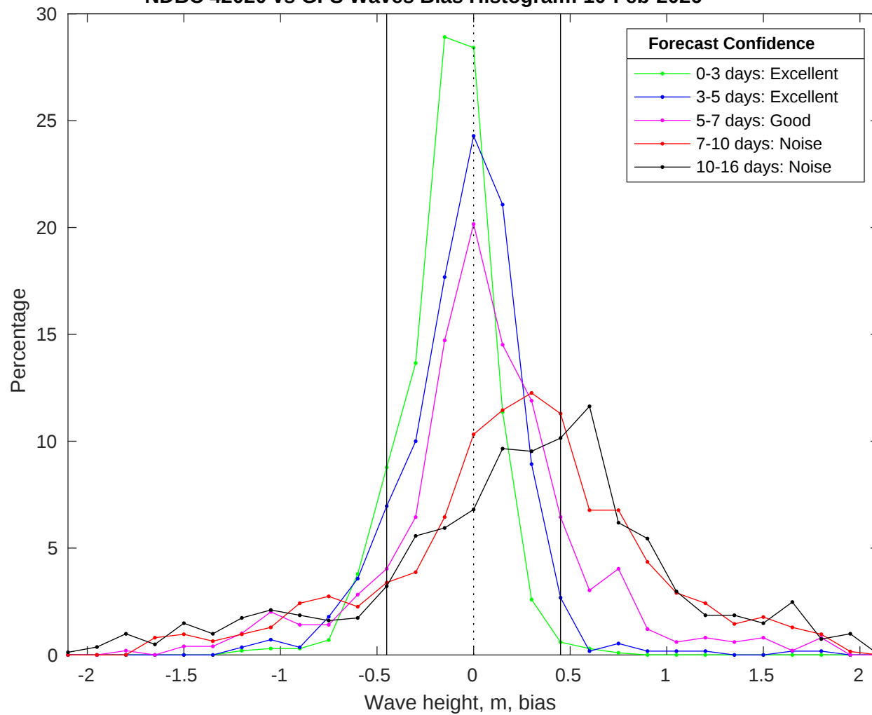
NDBC 42020 vs GFS Waves Bias Histogram: 10-Feb-2026
