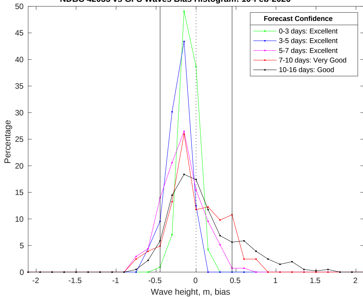
NDBC 42035 vs GFS Waves Bias Histogram: 10-Feb-2026
