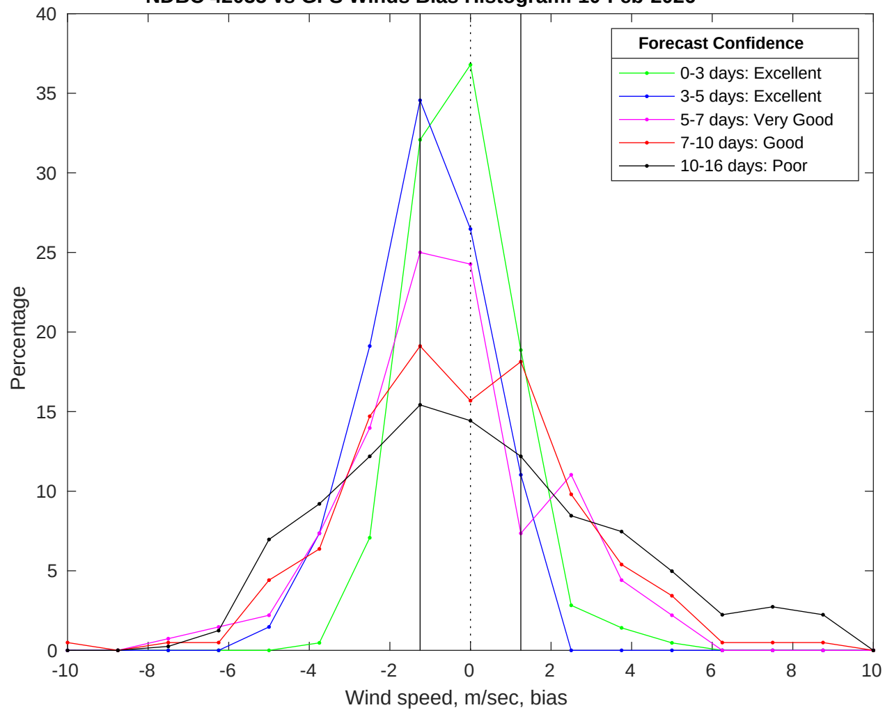
NDBC 42035 vs GFS Winds Bias Histogram: 10-Feb-2026
