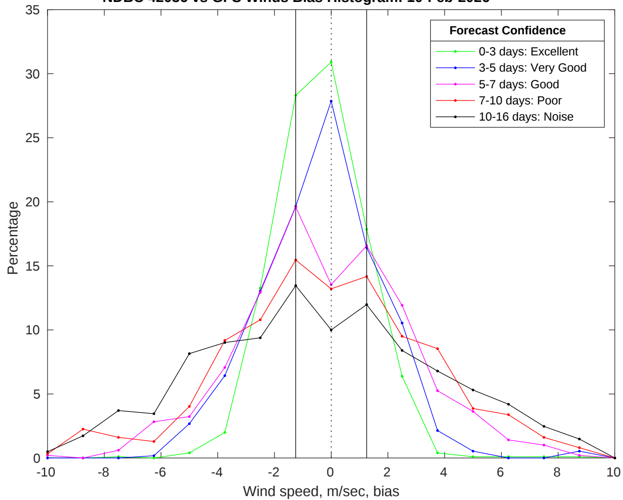
NDBC 42036 vs GFS Winds Bias Histogram: 10-Feb-2026
