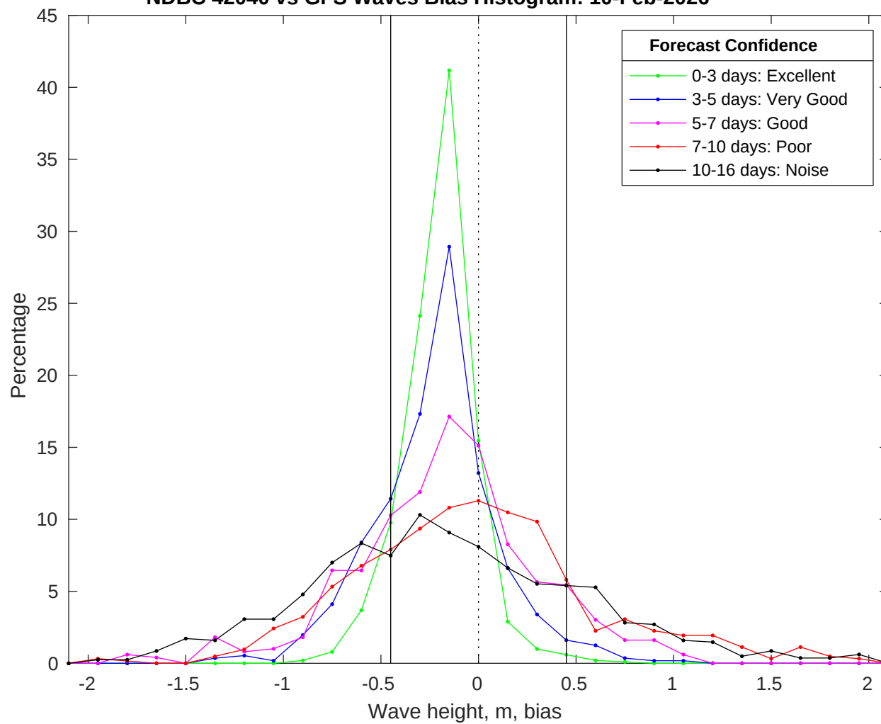
NDBC 42040 vs GFS Waves Bias Histogram: 10-Feb-2026
