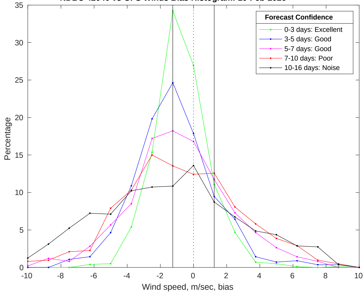
NDBC 42040 vs GFS Winds Bias Histogram: 10-Feb-2026
