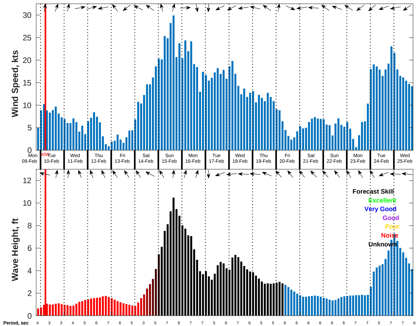
Wind & Wave Forecast for NDBC 42058 from 09-Feb-2026 20:00:00 to 25-Feb-2026 20:00:00
