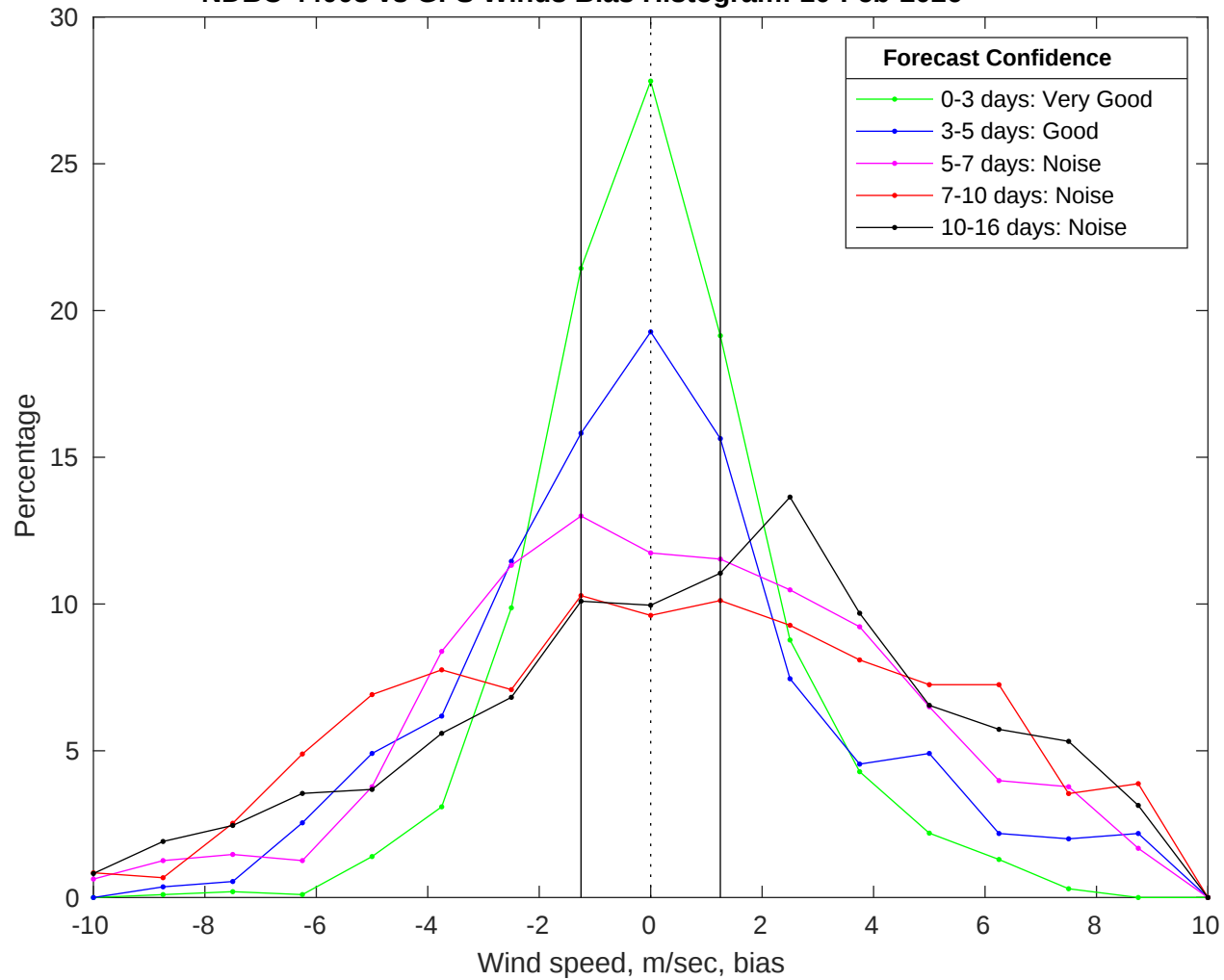
NDBC 44008 vs GFS Winds Bias Histogram: 10-Feb-2026
