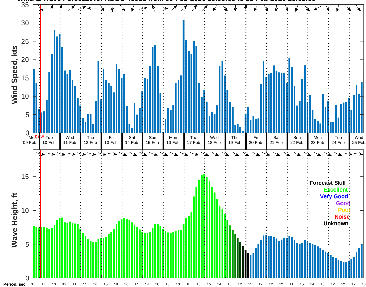
Wind & Wave Forecast for NDBC 46011 from 09-Feb-2026 16:00:00 to 25-Feb-2026 16:00:00
