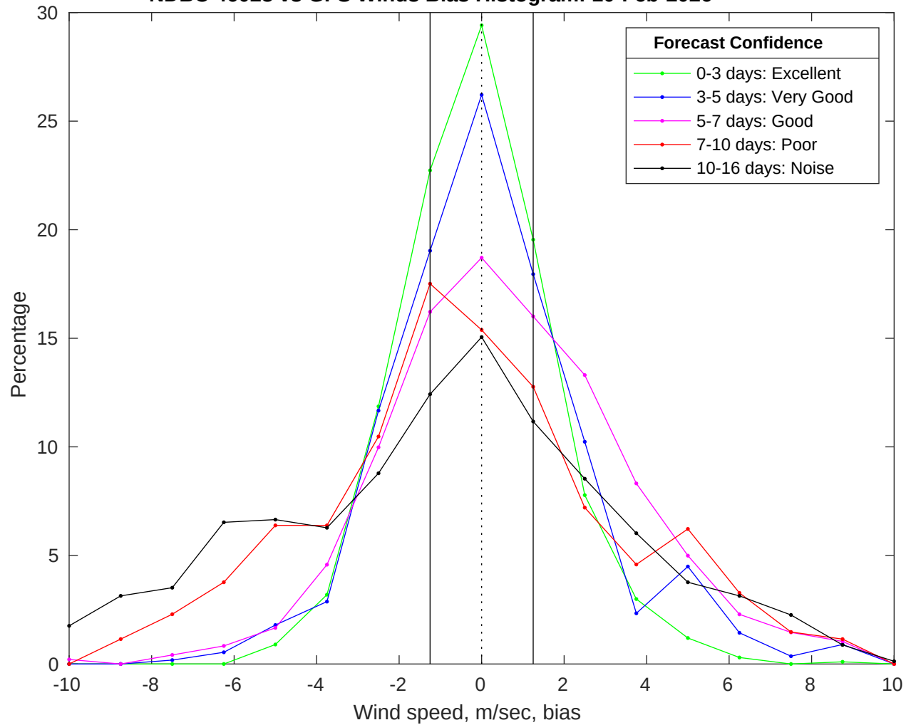
NDBC 46028 vs GFS Winds Bias Histogram: 10-Feb-2026
