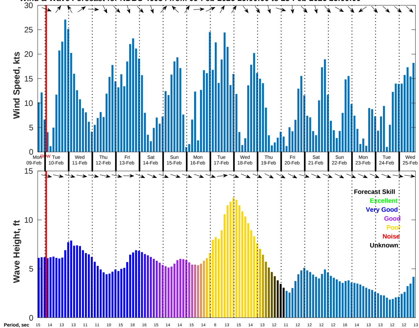
Wind & Wave Forecast for NDBC 46054 from 09-Feb-2026 16:00:00 to 25-Feb-2026 16:00:00
