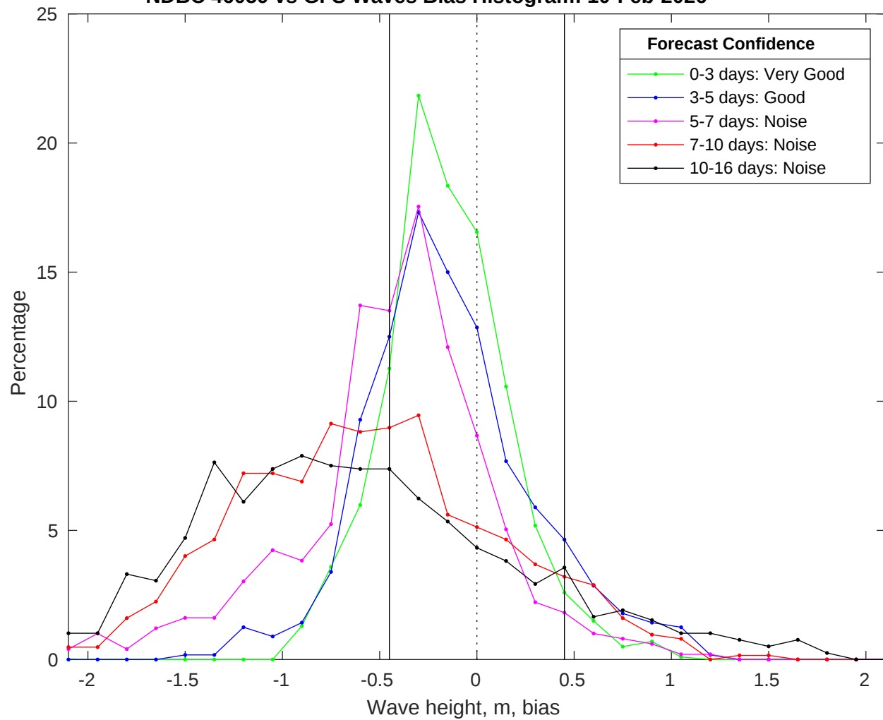
NDBC 46059 vs GFS Waves Bias Histogram: 10-Feb-2026
