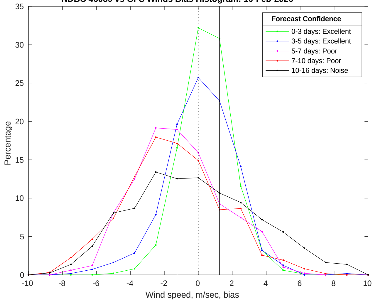
NDBC 46059 vs GFS Winds Bias Histogram: 10-Feb-2026
