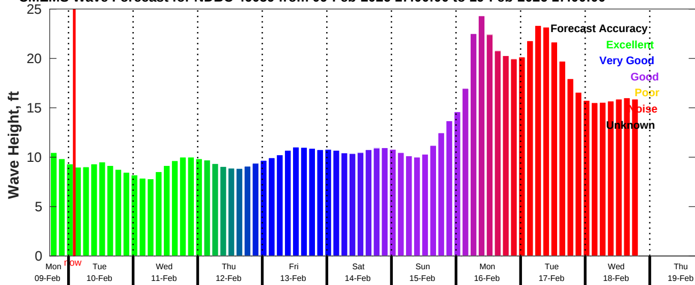
CMEMS Wave Forecast for NDBC 46059 from 09-Feb-2026 17:00:00 to 19-Feb-2026 17:00:00
