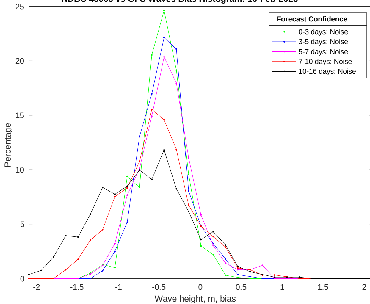
NDBC 46069 vs GFS Waves Bias Histogram: 10-Feb-2026
