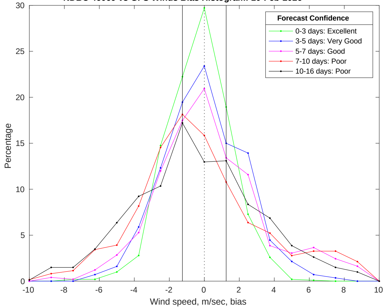
NDBC 46069 vs GFS Winds Bias Histogram: 10-Feb-2026
