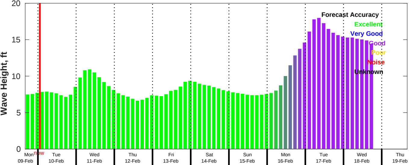
CMEMS Wave Forecast for NDBC 46069 from 09-Feb-2026 16:00:00 to 19-Feb-2026 16:00:00
