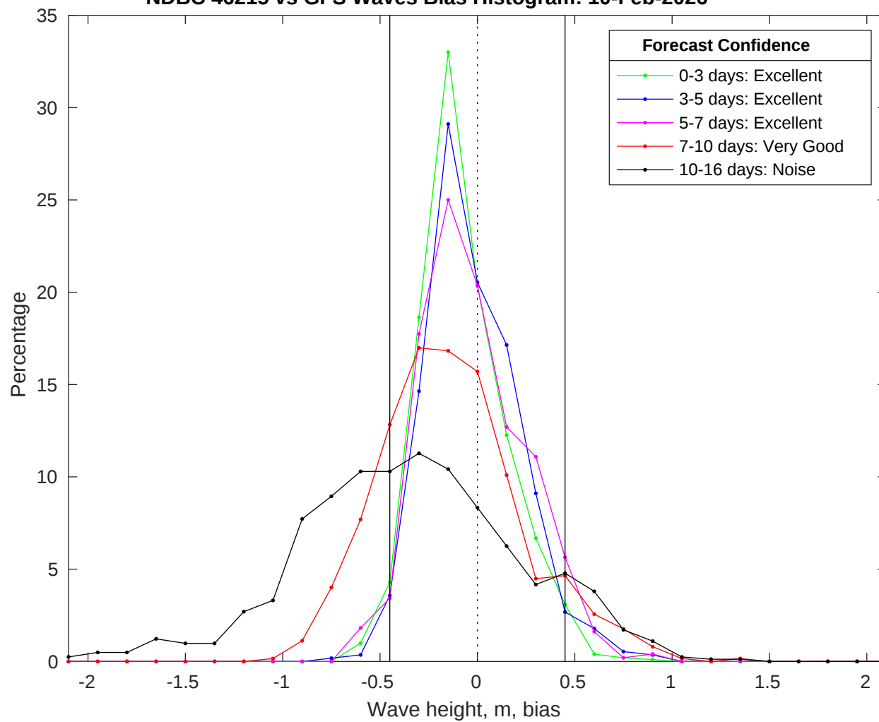
NDBC 46215 vs GFS Waves Bias Histogram: 10-Feb-2026
