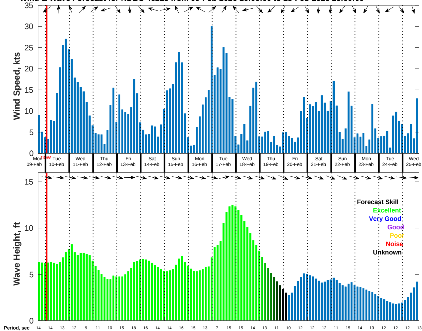
Wind & Wave Forecast for NDBC 46215 from 09-Feb-2026 16:00:00 to 25-Feb-2026 16:00:00
