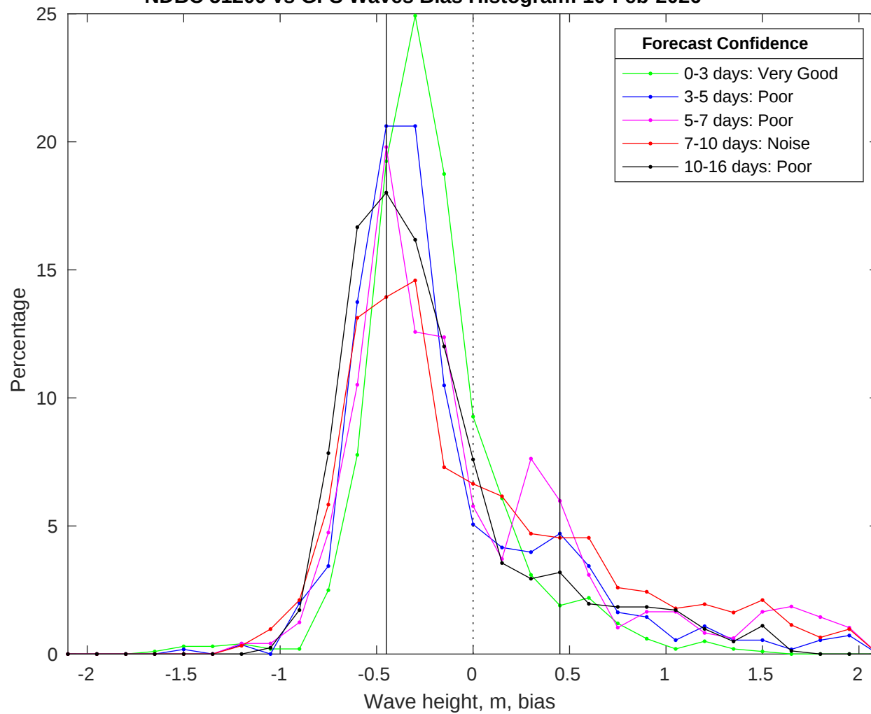
NDBC 51209 vs GFS Waves Bias Histogram: 10-Feb-2026
