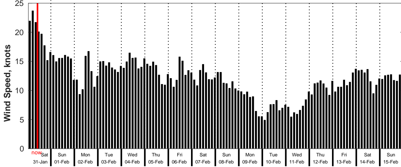
GFS Wind Speed Forecast for NDBC 51209 from 31-Jan-2026 01:00:00 to 16-Feb-2026 01:00:00
